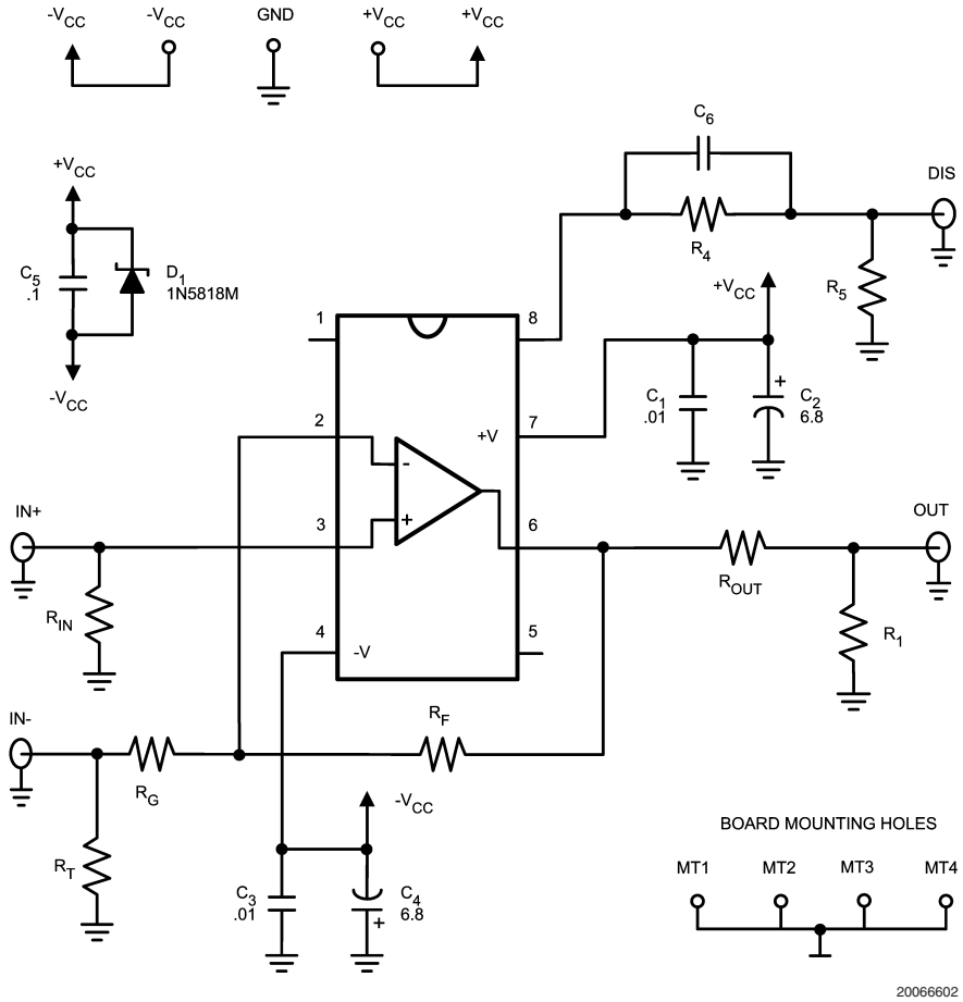
FIGURE 2. SOIC Schematic
