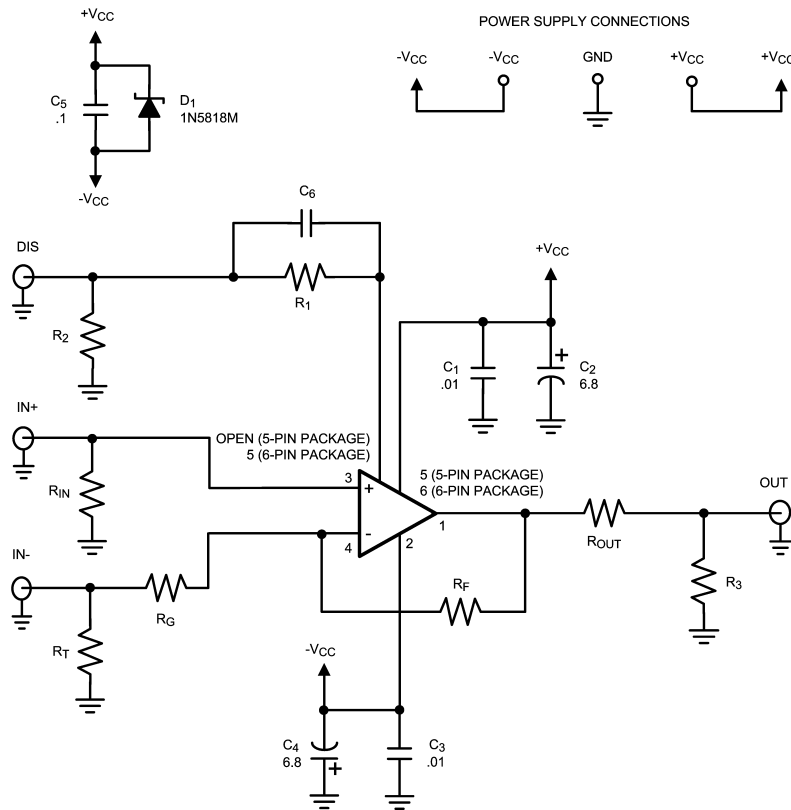
FIGURE 1. SOT and SC70 Schematic
